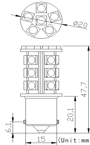
1156 LED bulb 5050*27PCS Flat foot bronze head 8-30V White
